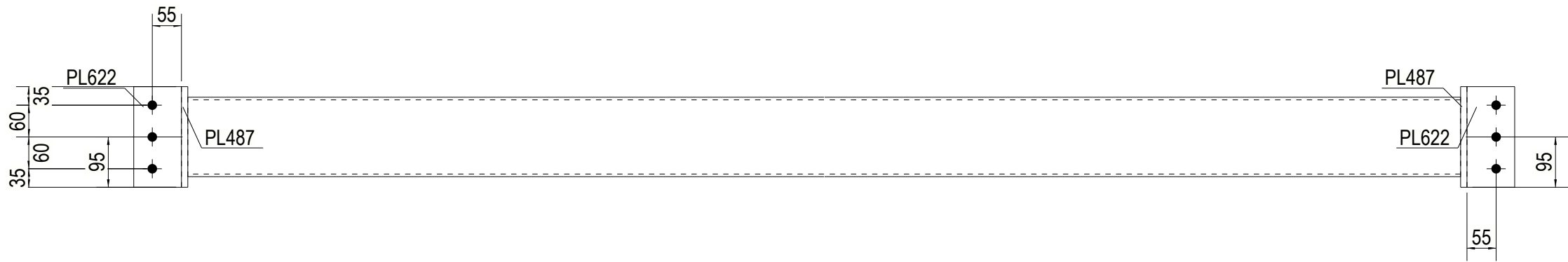
TOP VIEW
